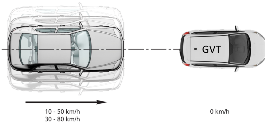
Figure 6a: CCRs scenario
