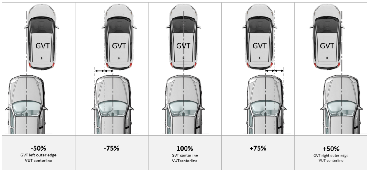
Figure 3: Lateral Overlap examples
