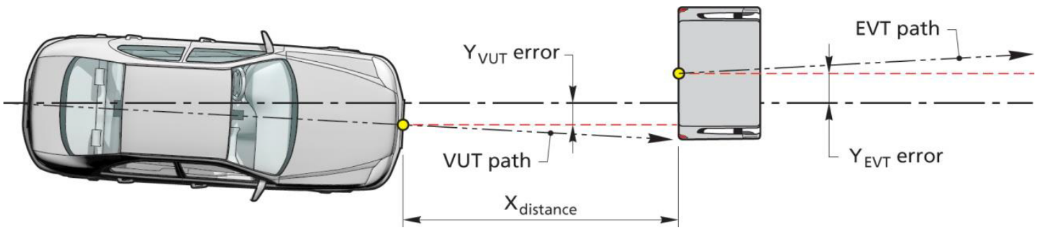
Figure 2: Lateral path error
